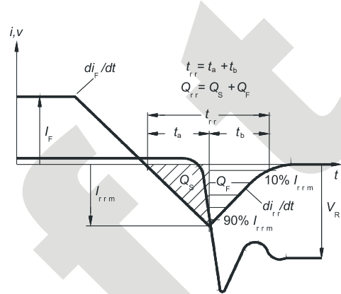
Figure C. Definition of diodes switching characteristics
