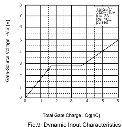
Fig.9 Dynamic Input Characteristics
