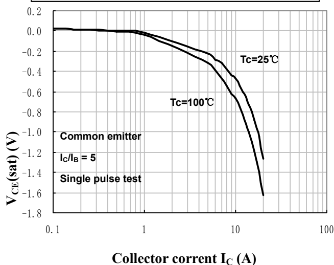
Saturation Voltage
