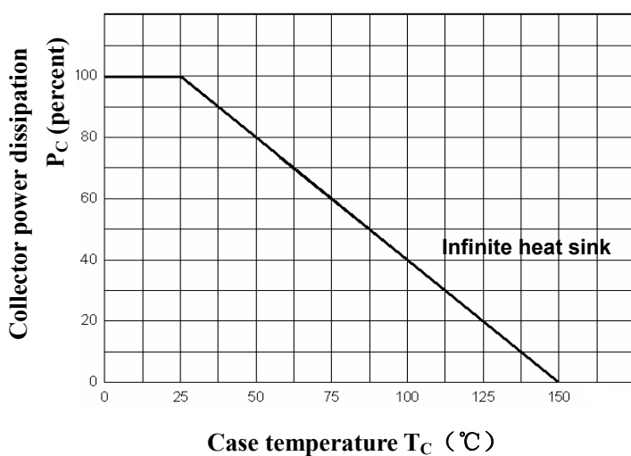
Power Derating
