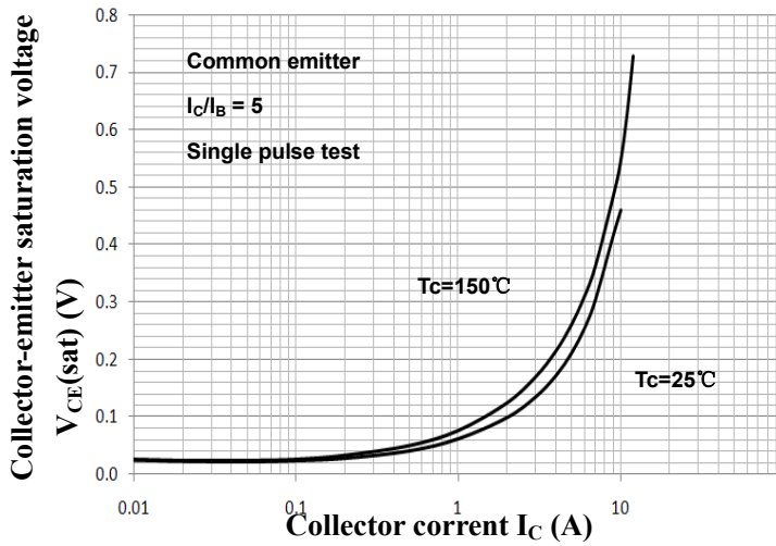
Saturation Voltage
