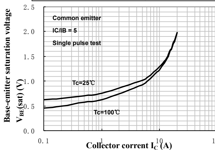
Saturation Voltage
