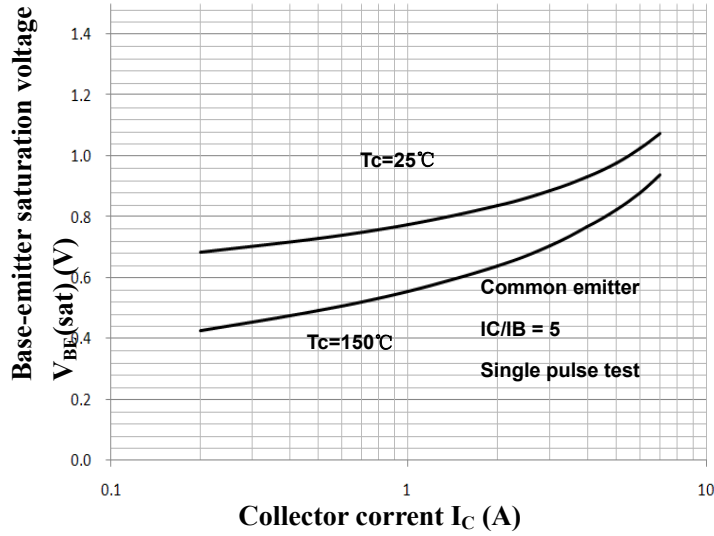
Saturation Voltage
