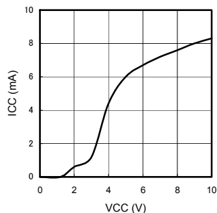
Fig.13 Circuit Current - Power Supply Voltage
