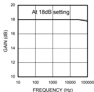
Fig.16 Current Gain - Frequency (BD3870FS, BD3873FS)
