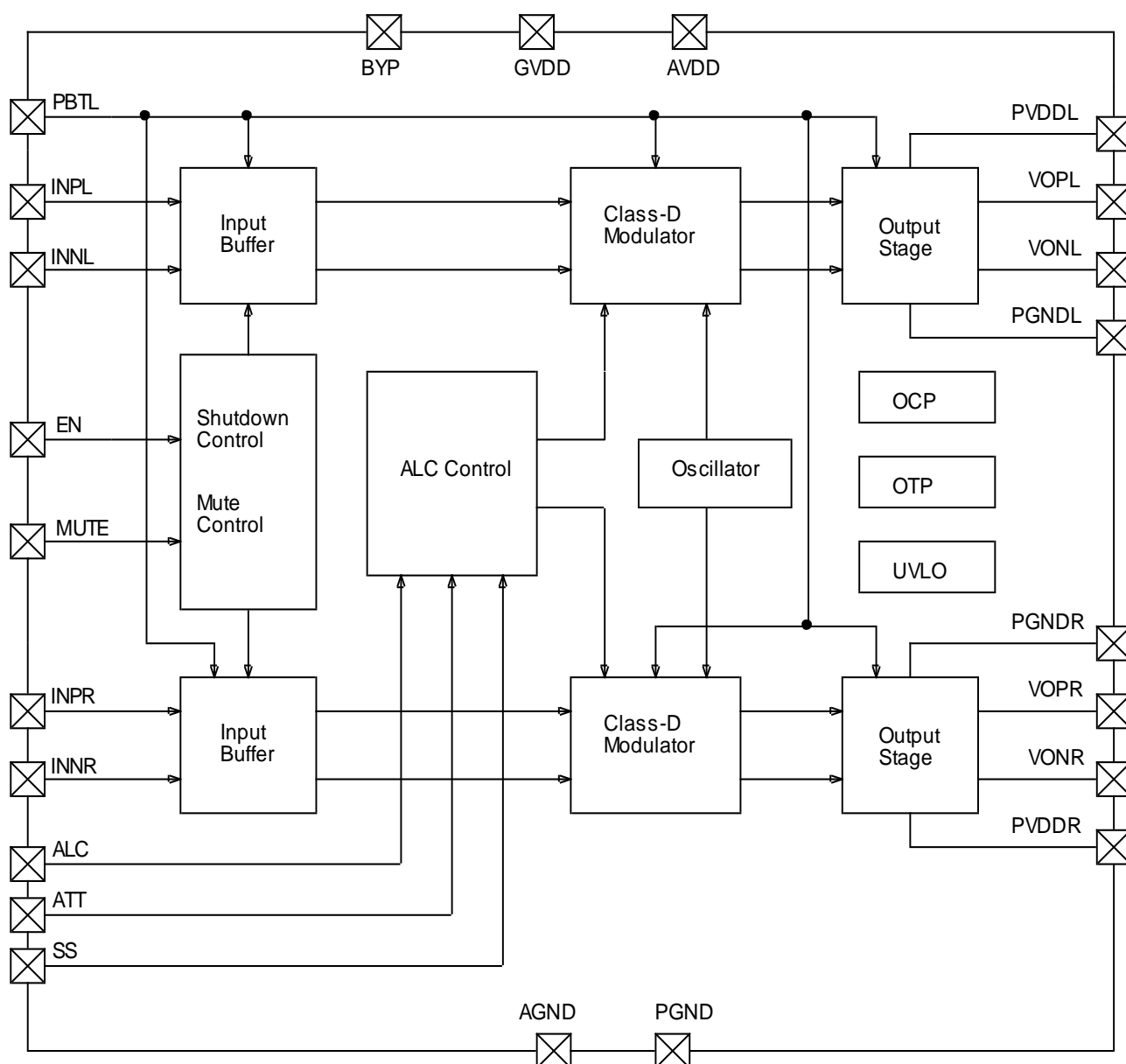
Figure 2: Simplified Functional Block Diagram of ft2725
