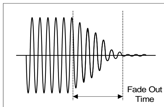
Figure 30: Fade-Out Waveform
