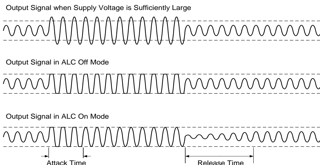
Figure 23: Automatic Level Control Diagram
