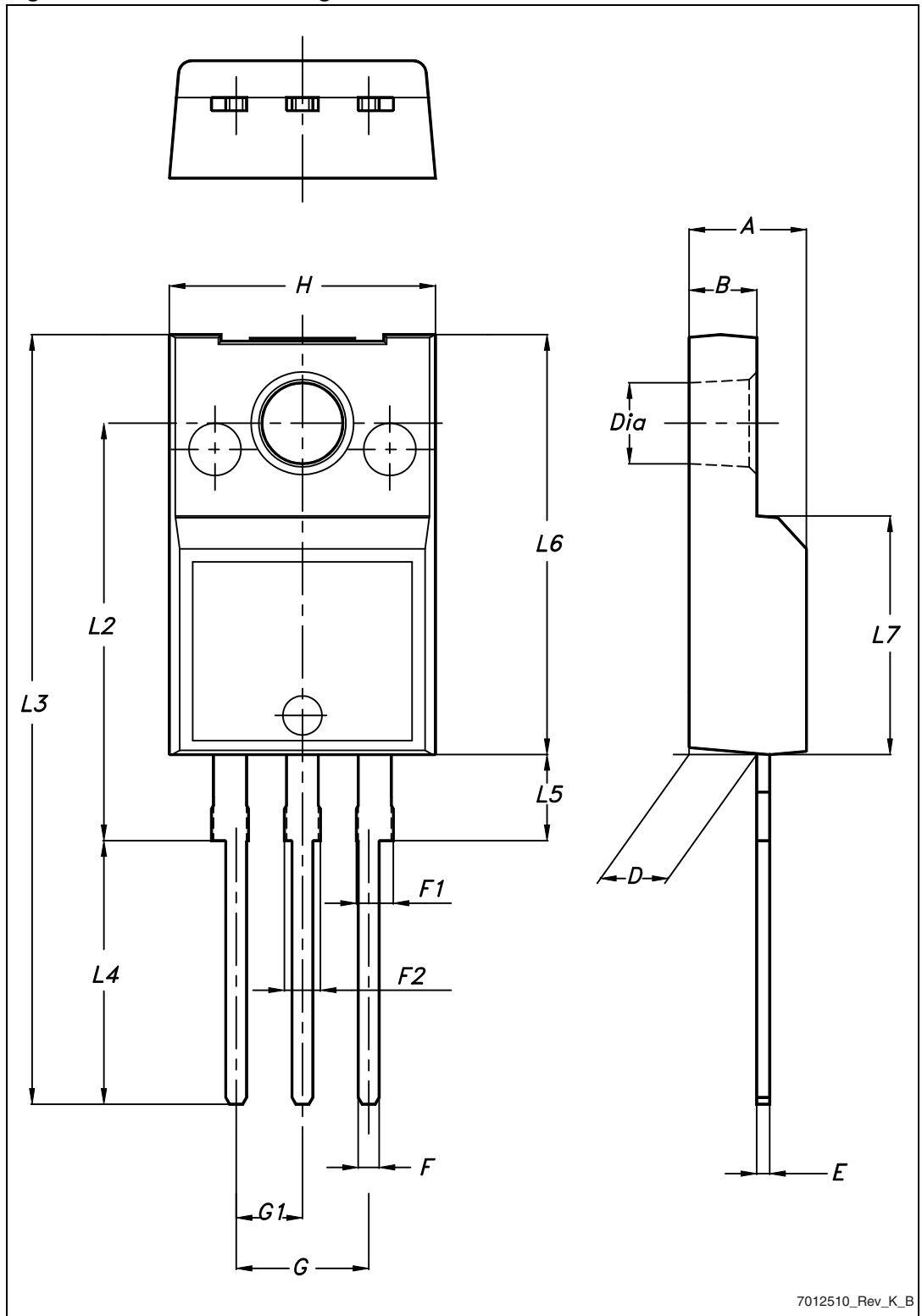
Figure 28. TO-220FP drawing
