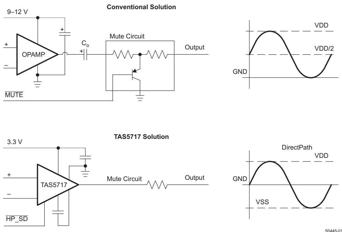
Figure 47. Conventional and DirectPath HP and Line Driver
