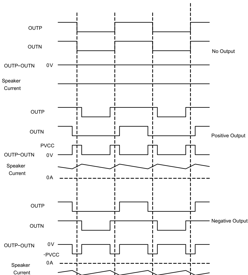
Figure 18. BD Mode Modulation
